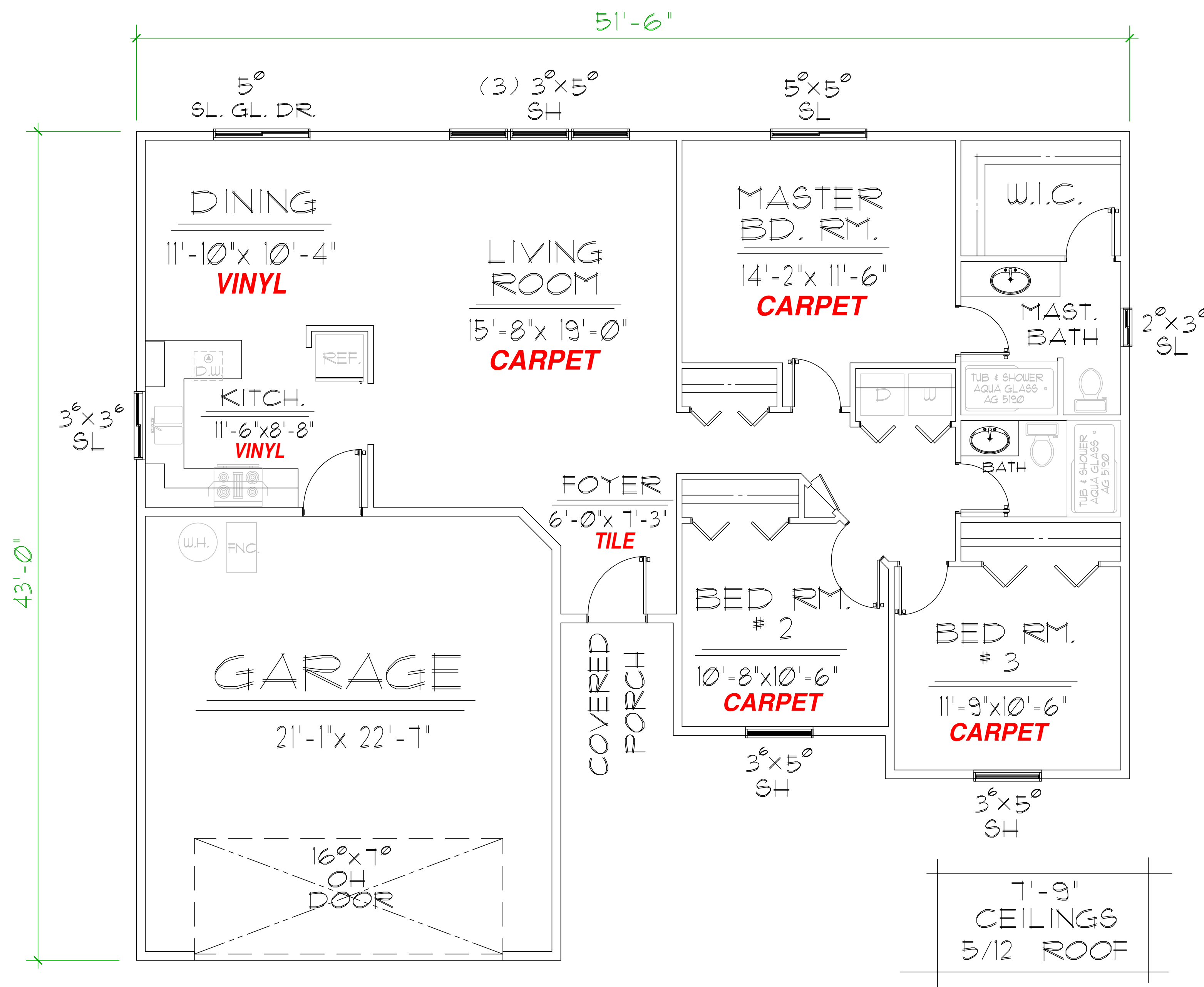
FLOOR PLAN
