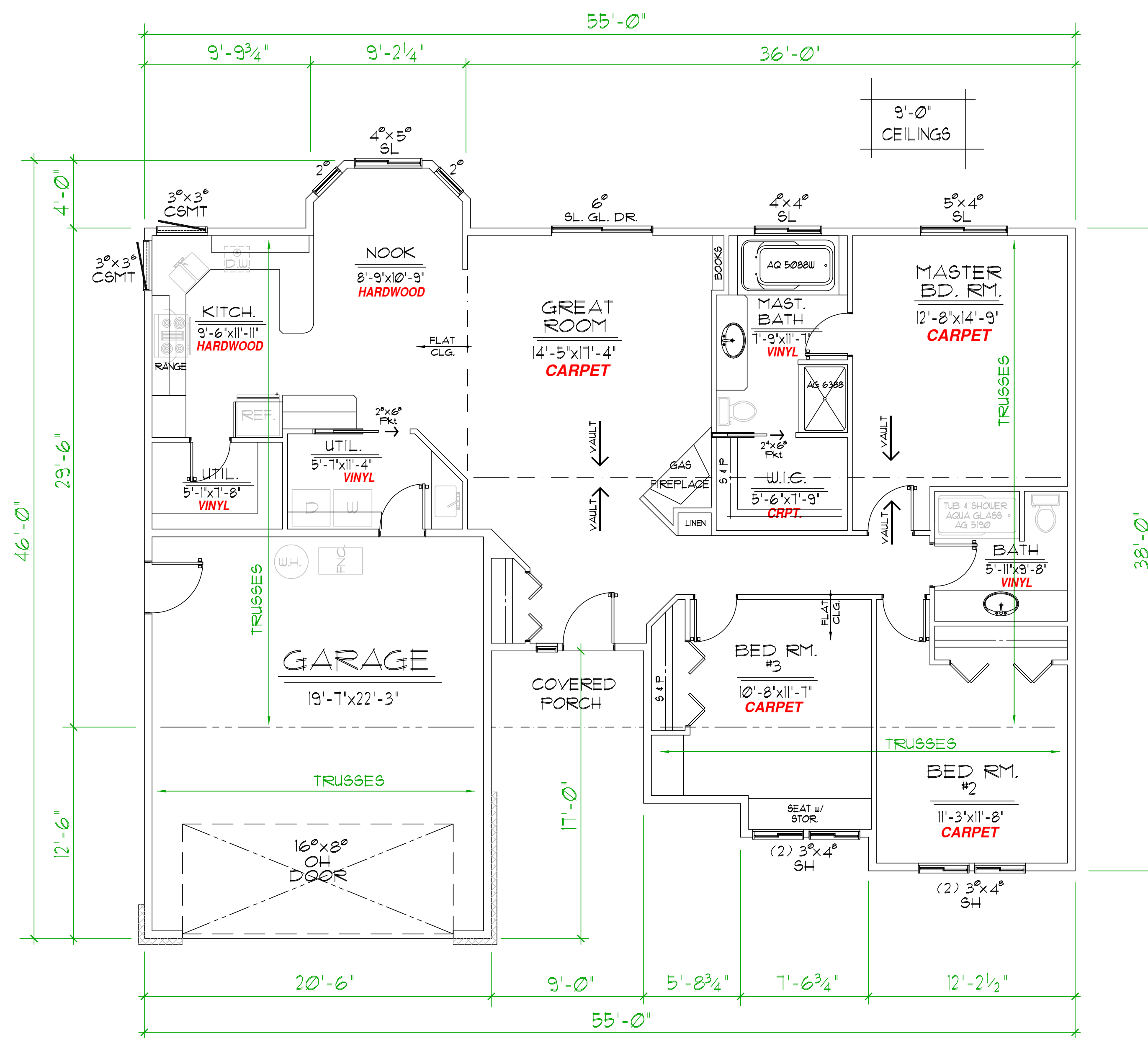
FLOOR PLAN
