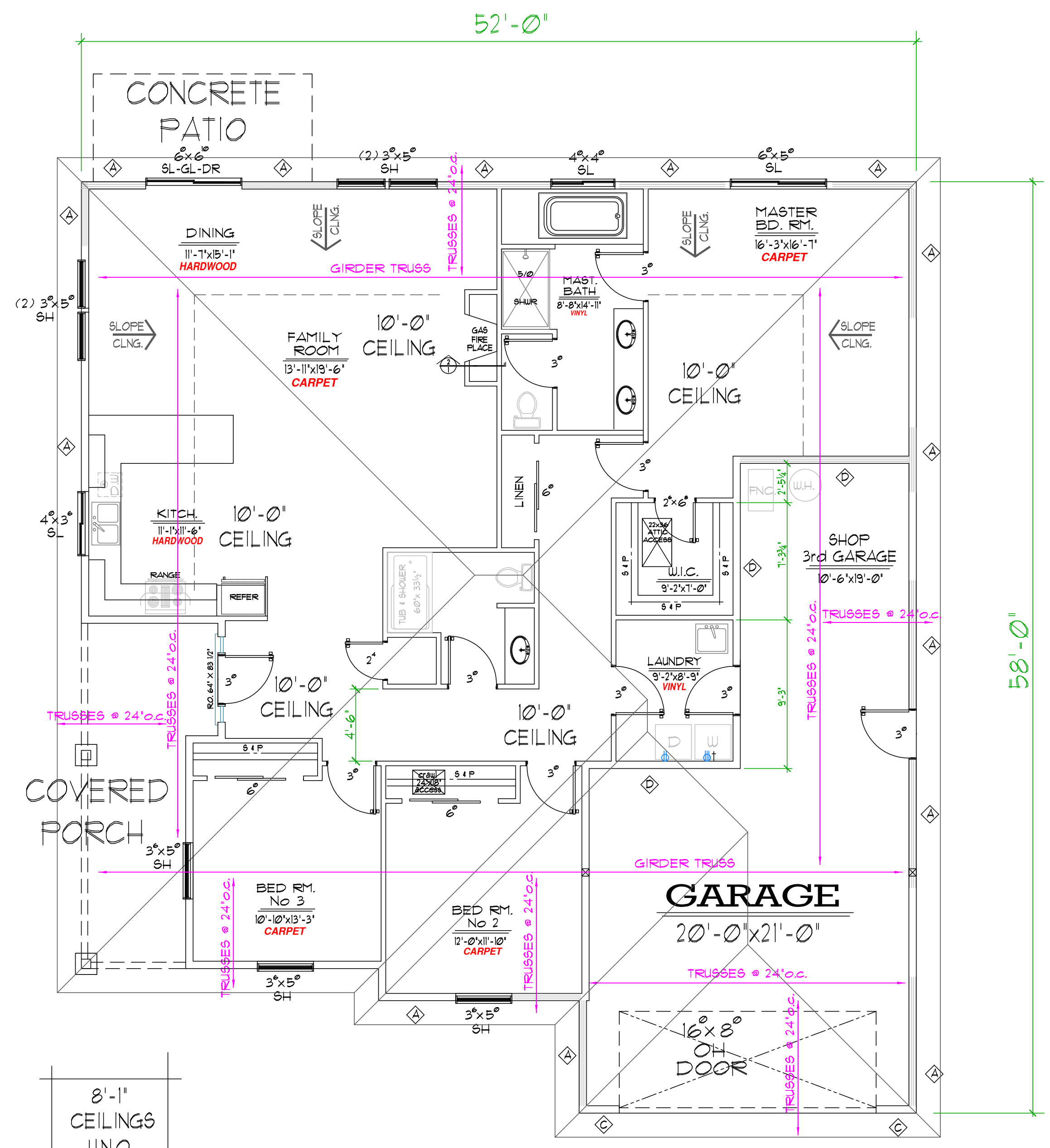
FLOOR PLAN 1958 SQ. FT GARAGE 650 SQ. FT
