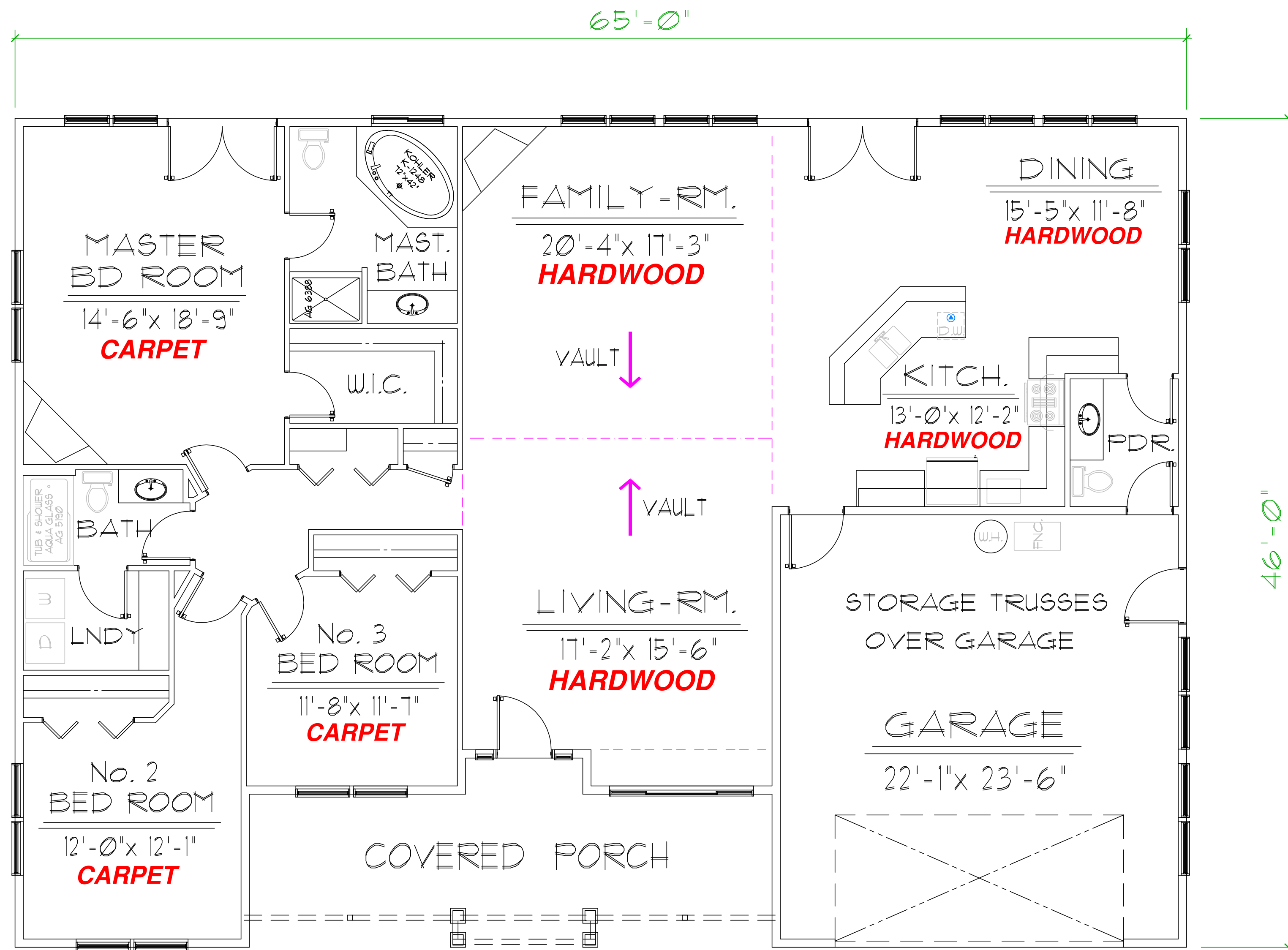
FLOOR PLAN
