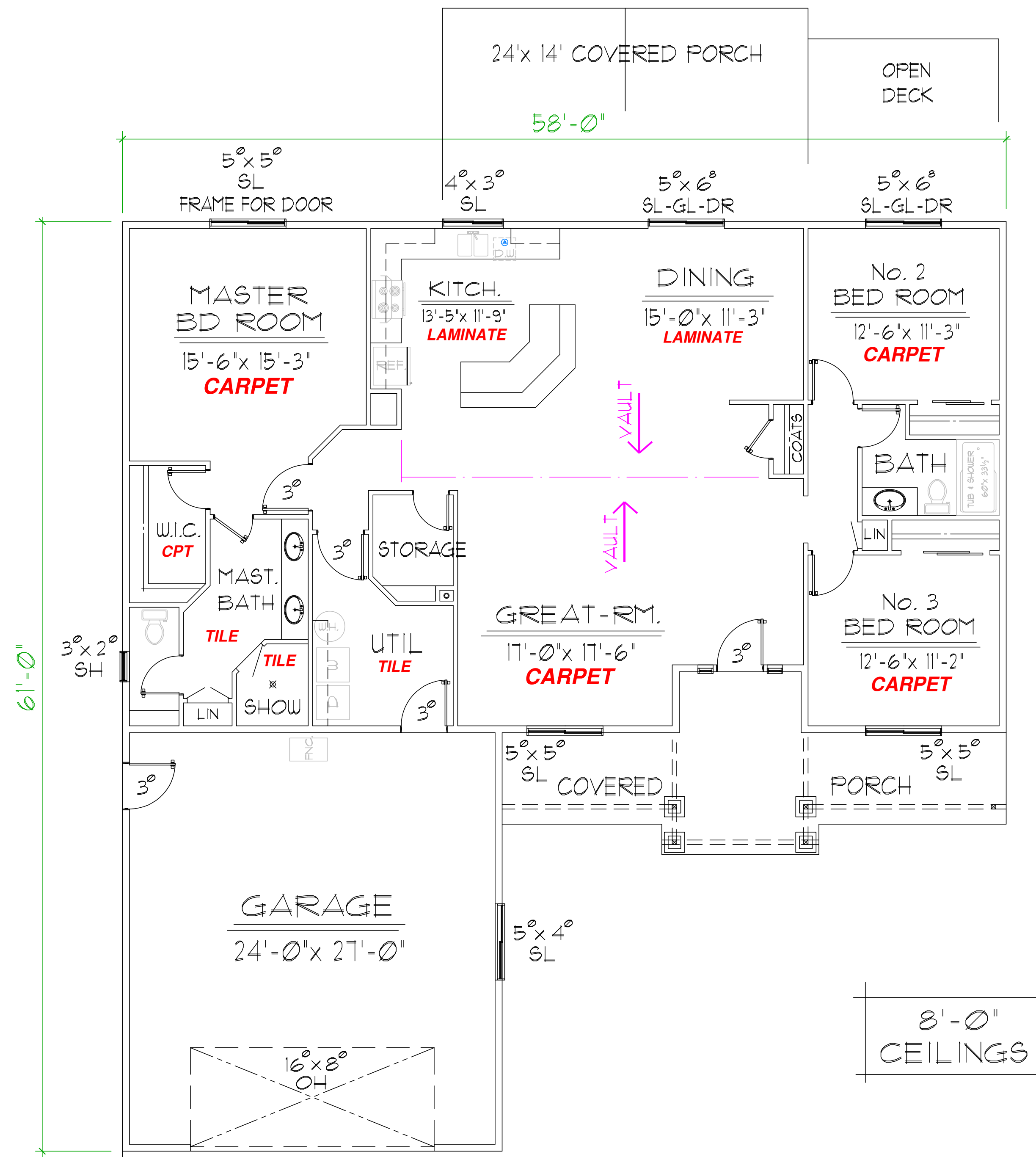
FLOOR PLAN
