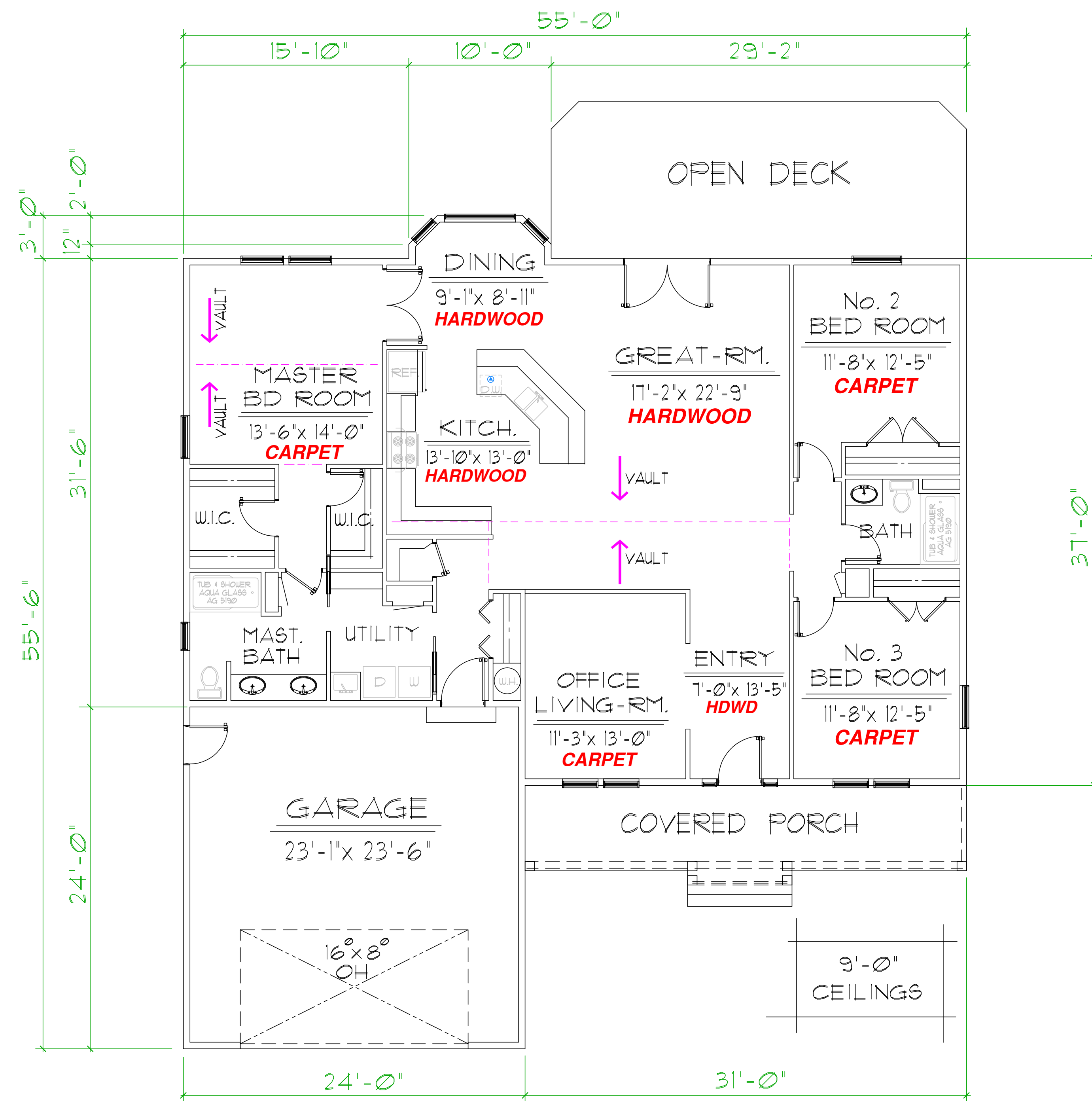
FLOOR PLAN
