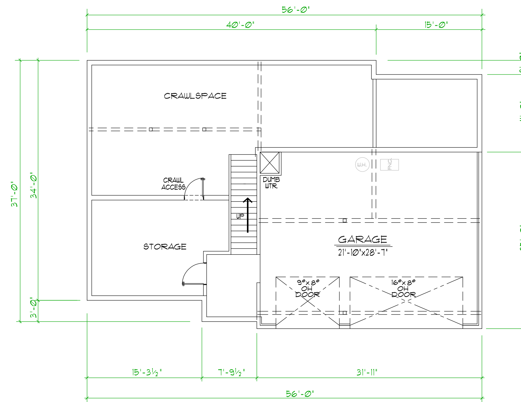
PLAN @ GARAGE
