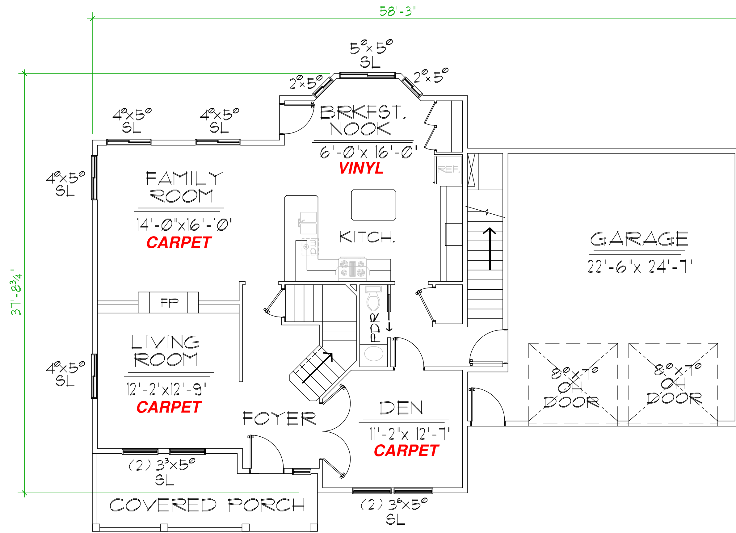
1st FLOOR PLAN
