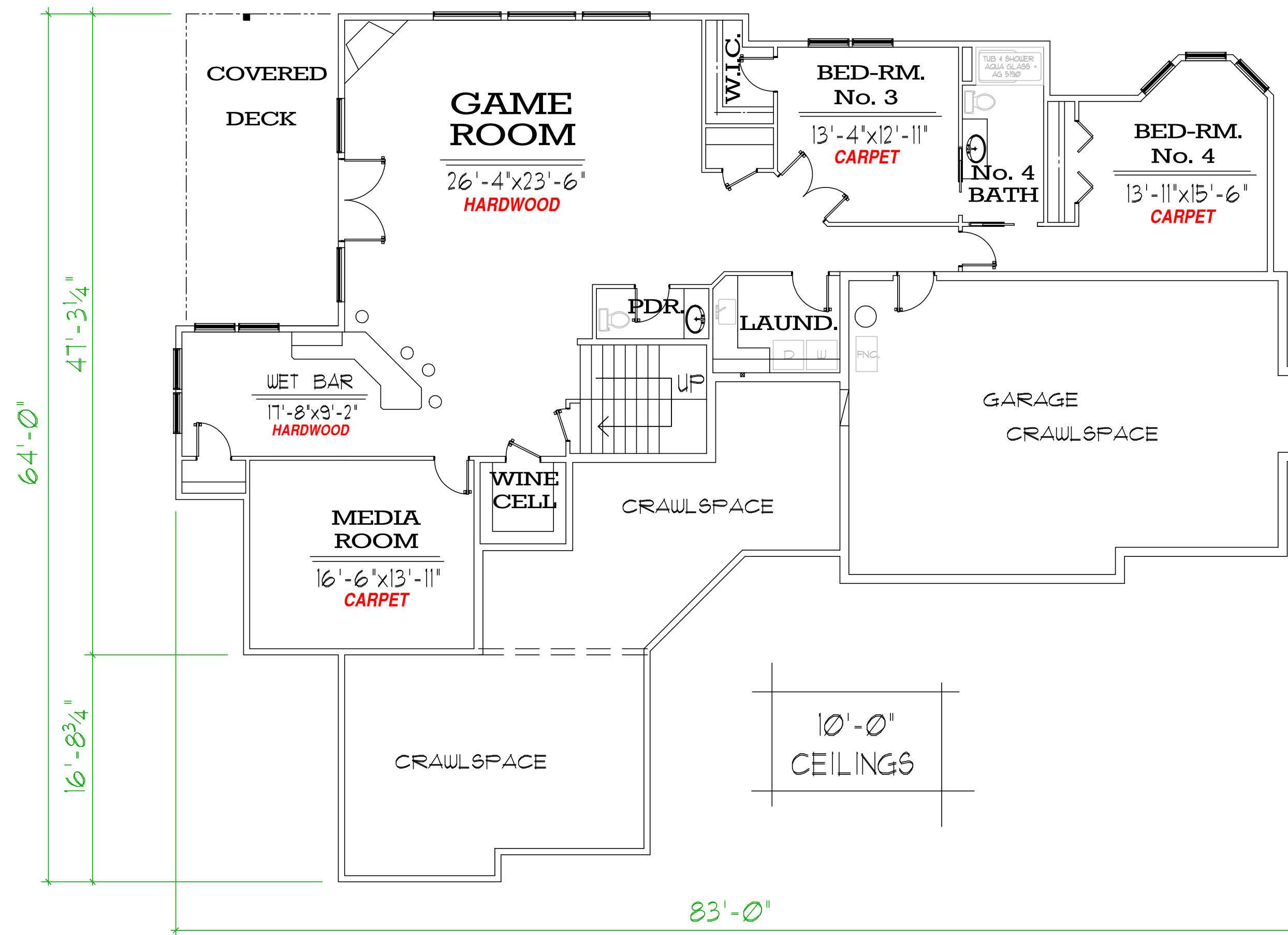
DAYLIGHT BASEMENT PLAN
