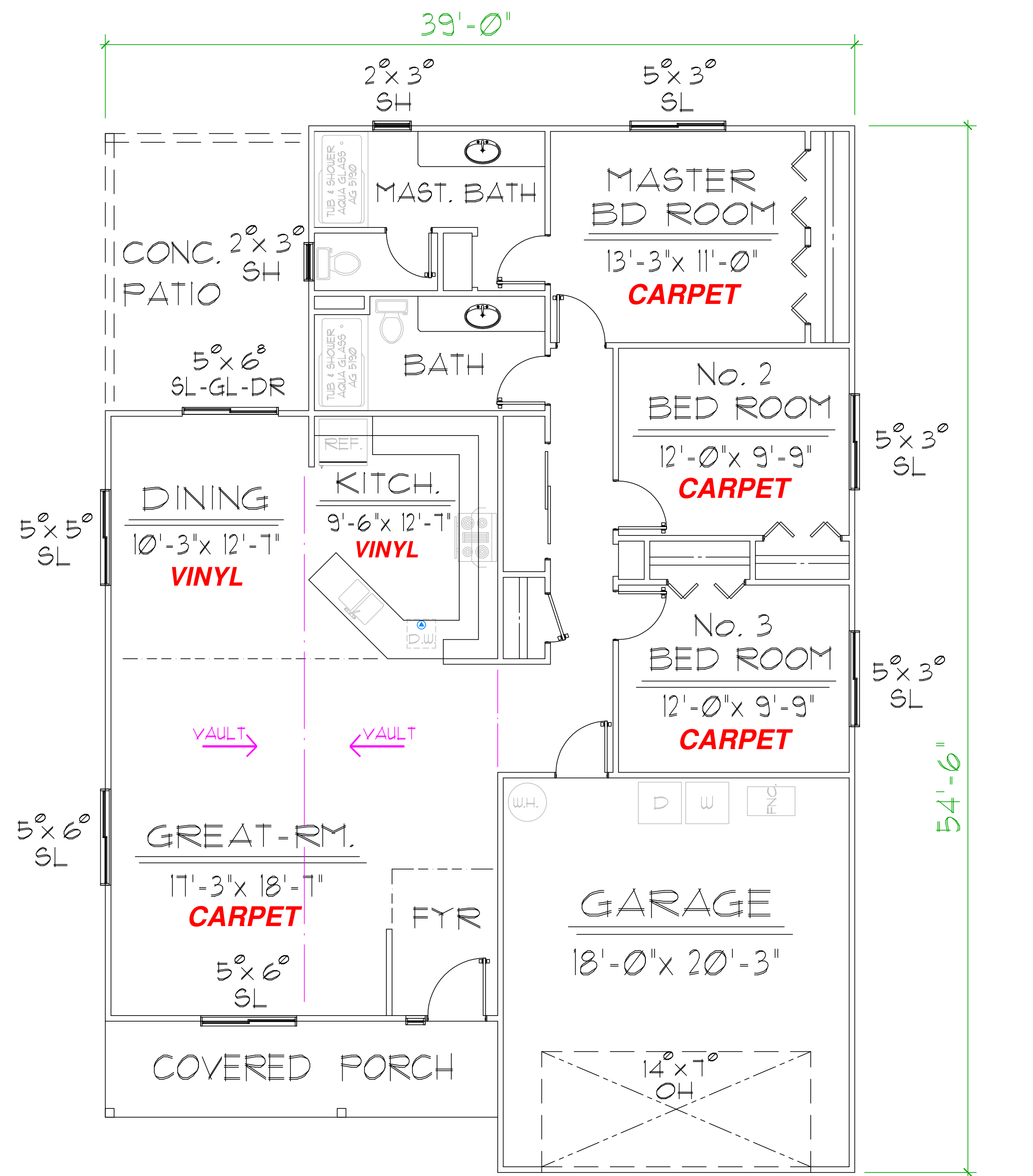
FLOOR PLAN
