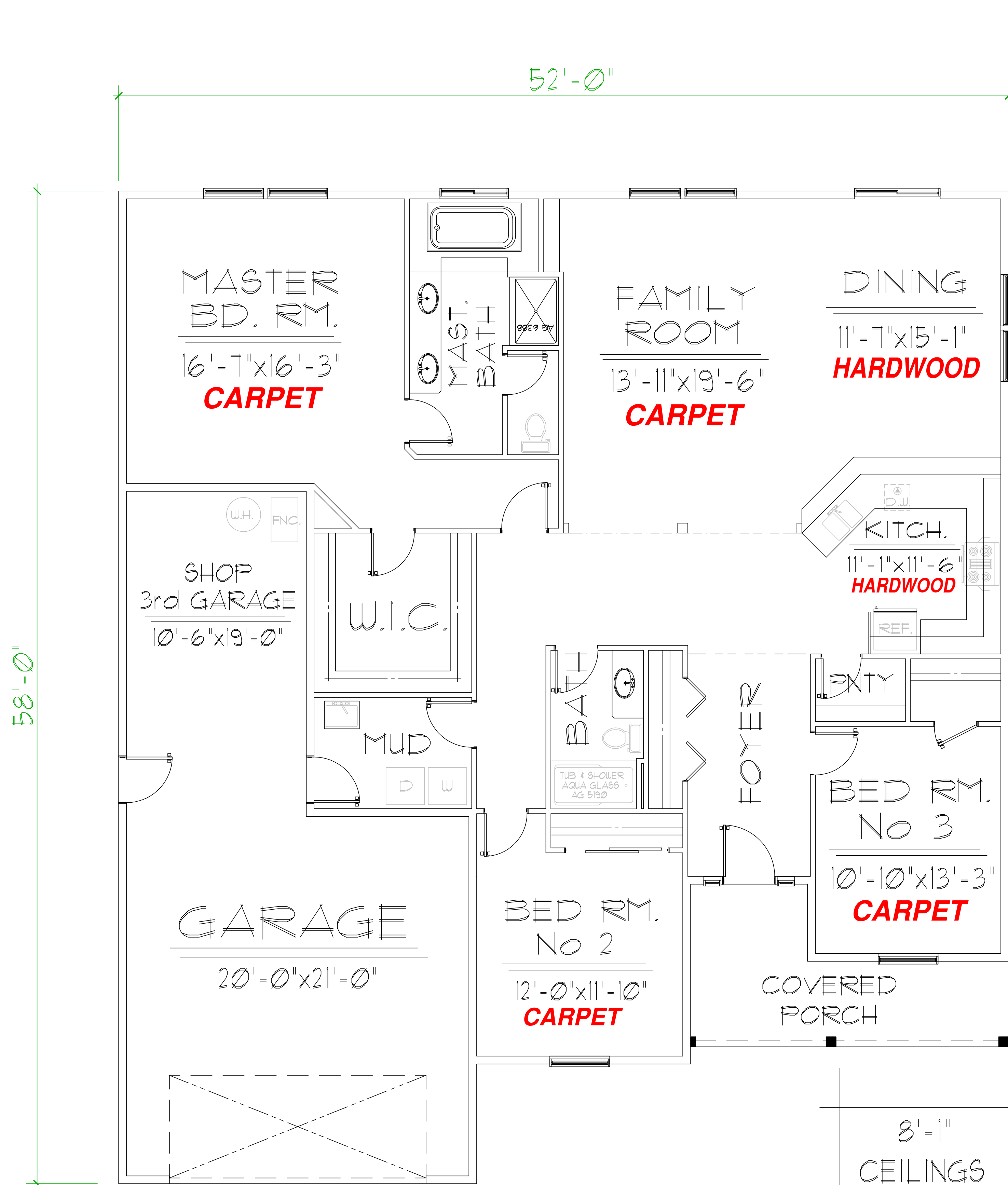
FLOOR PLAN
