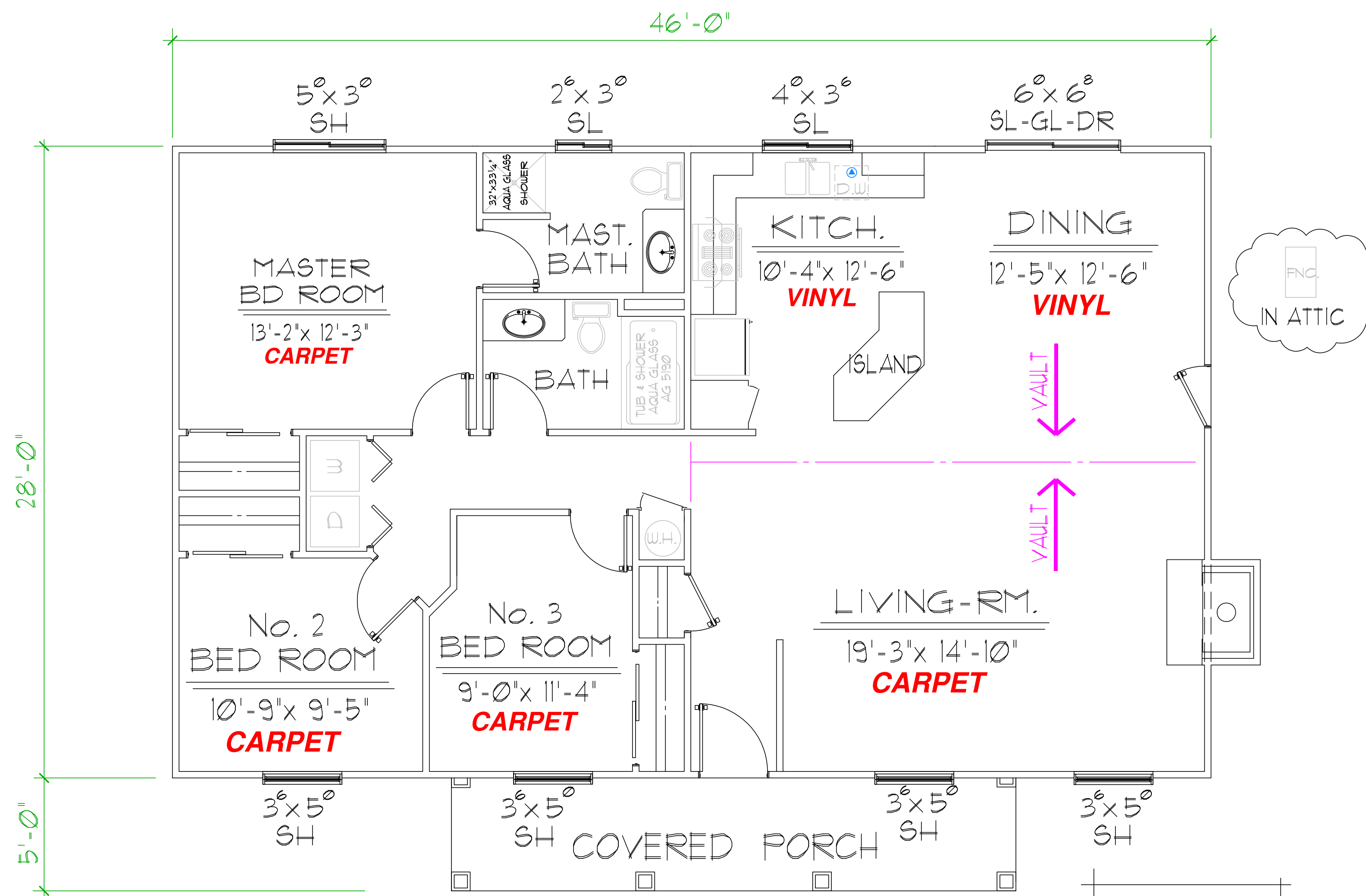
FLOOR PLAN
