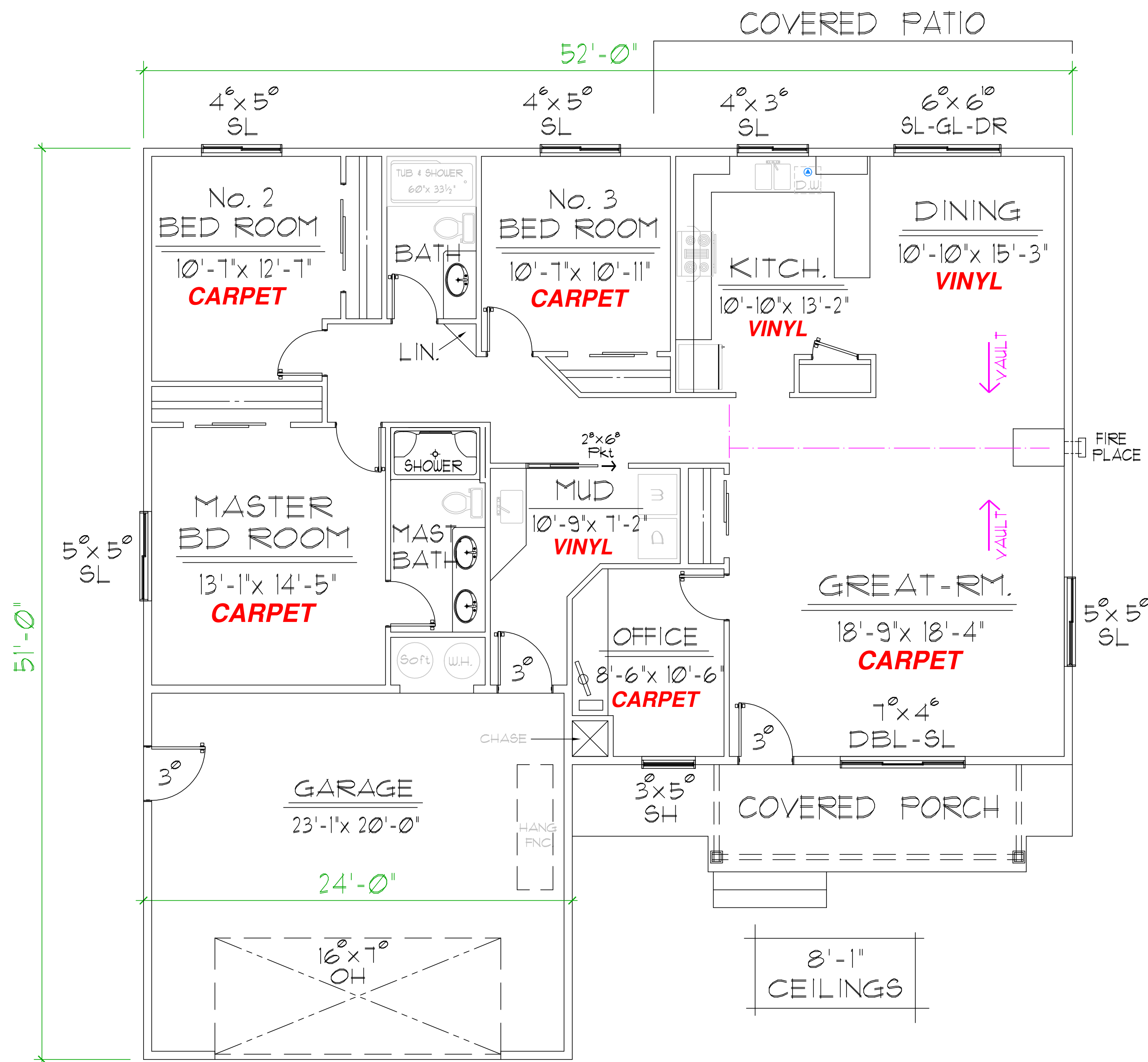
FLOOR PLAN
