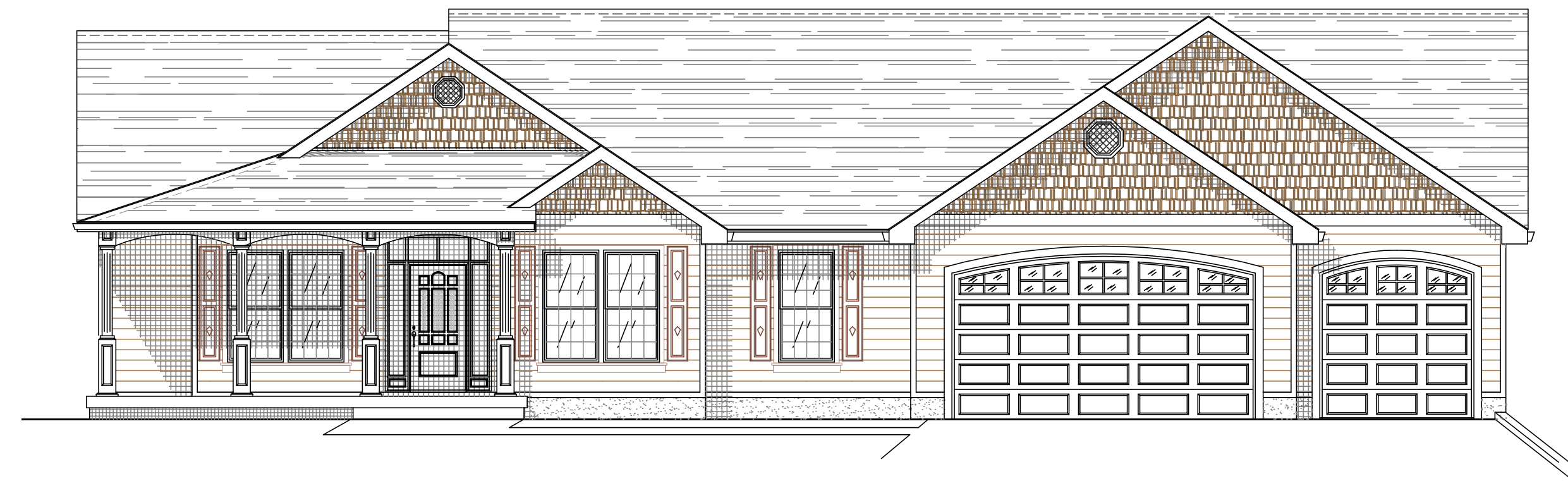
FRONT ELEV.
