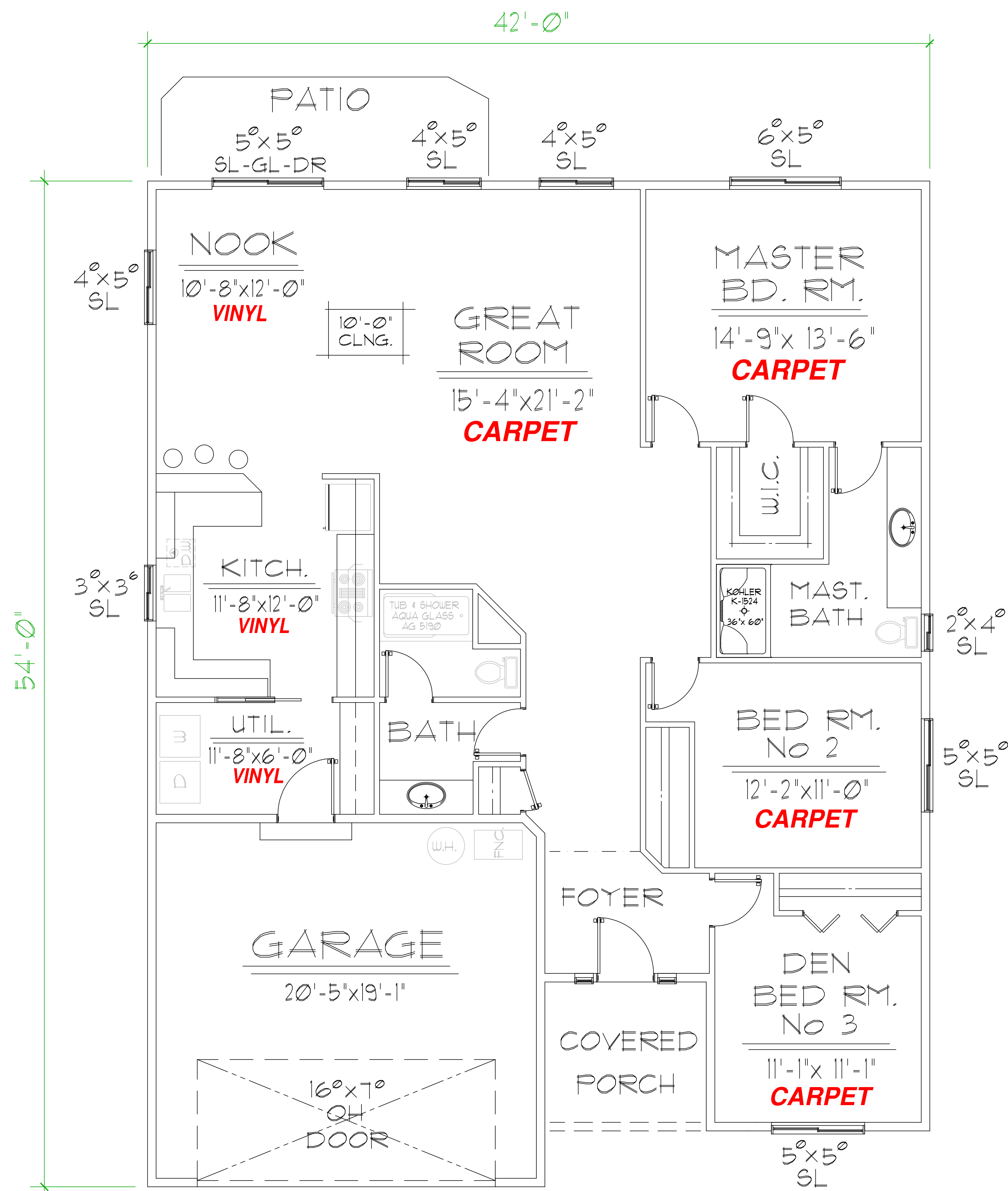
FLOOR PLAN
