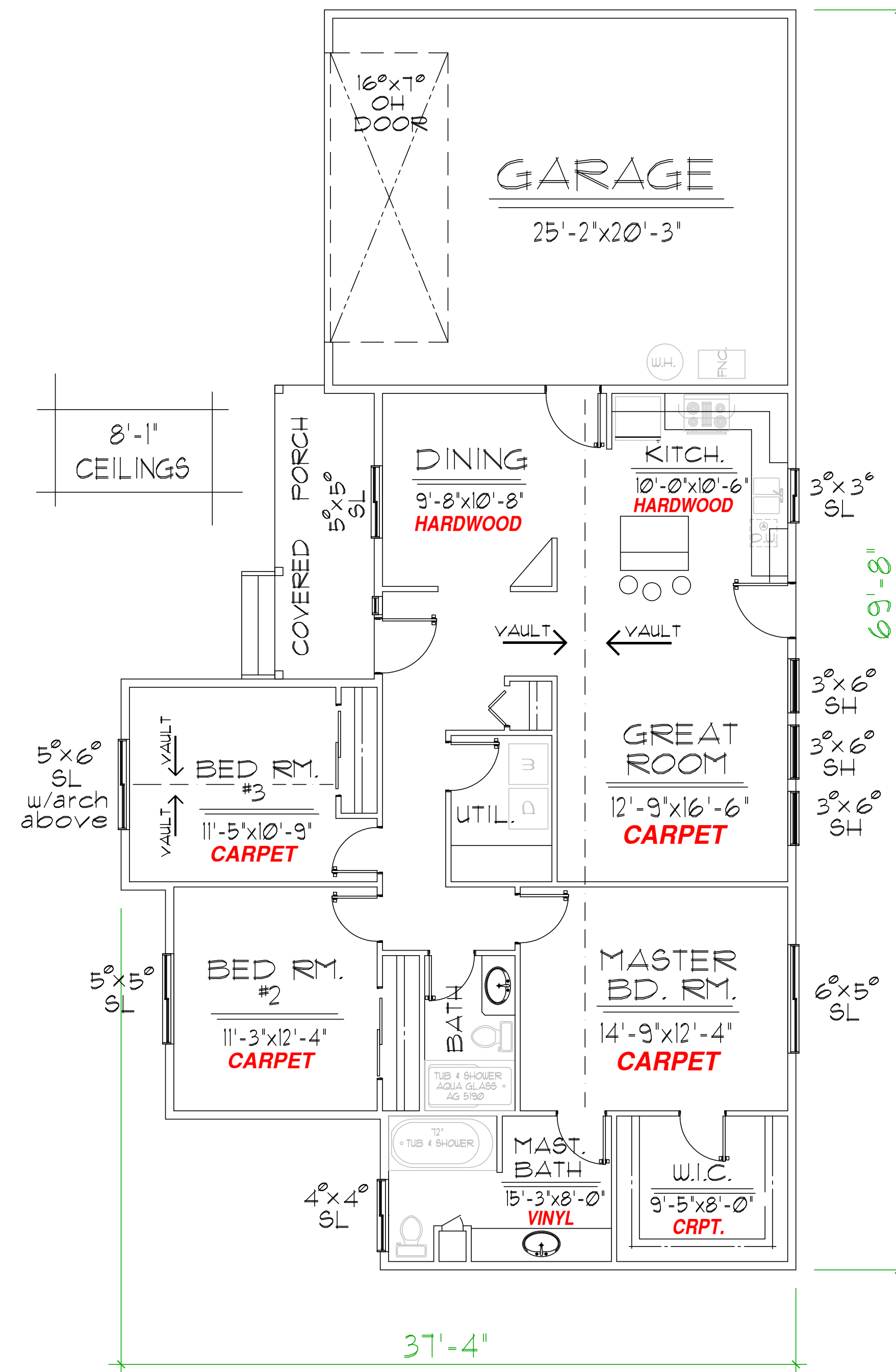
FLOOR PLAN
