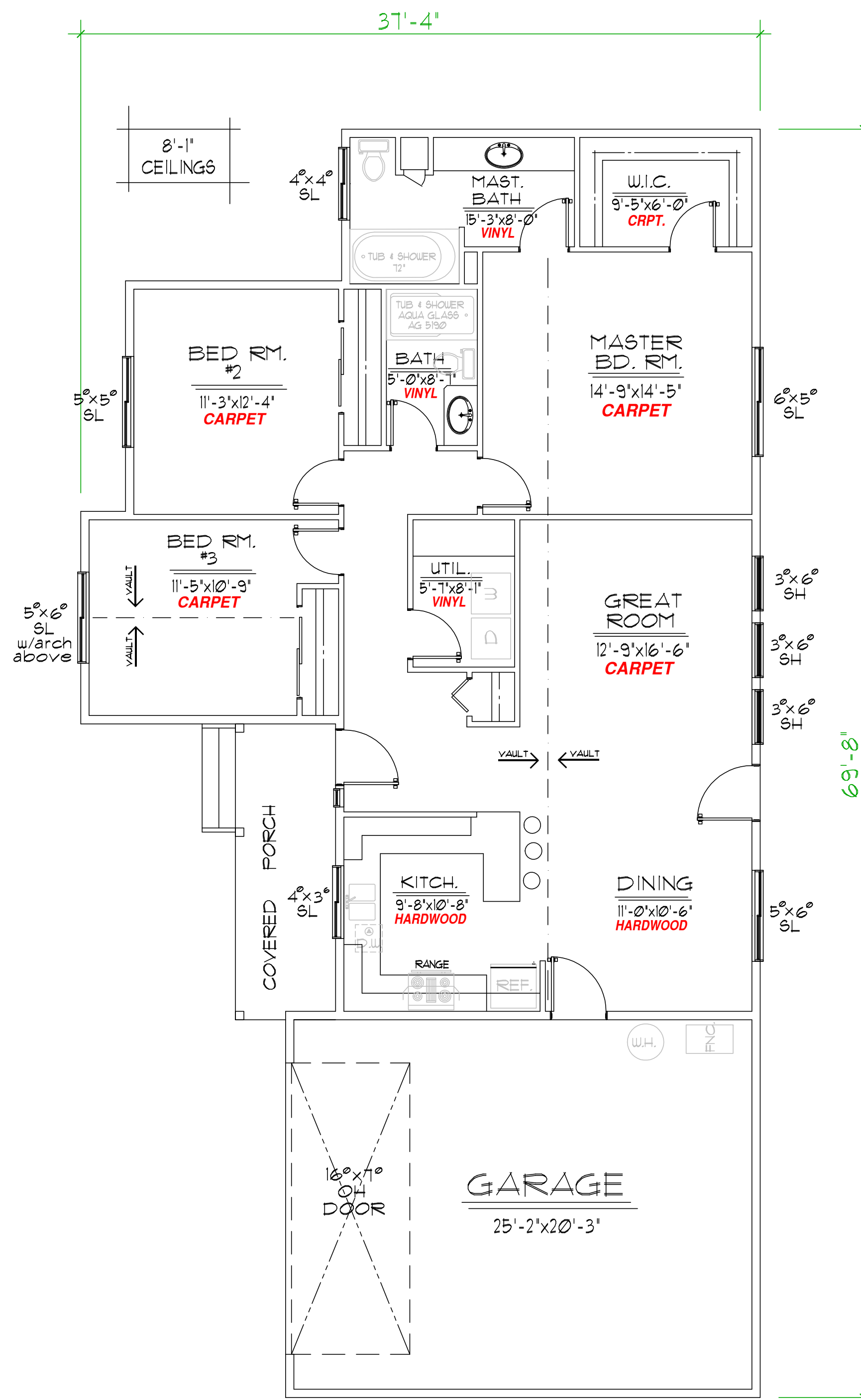
FLOOR PLAN
